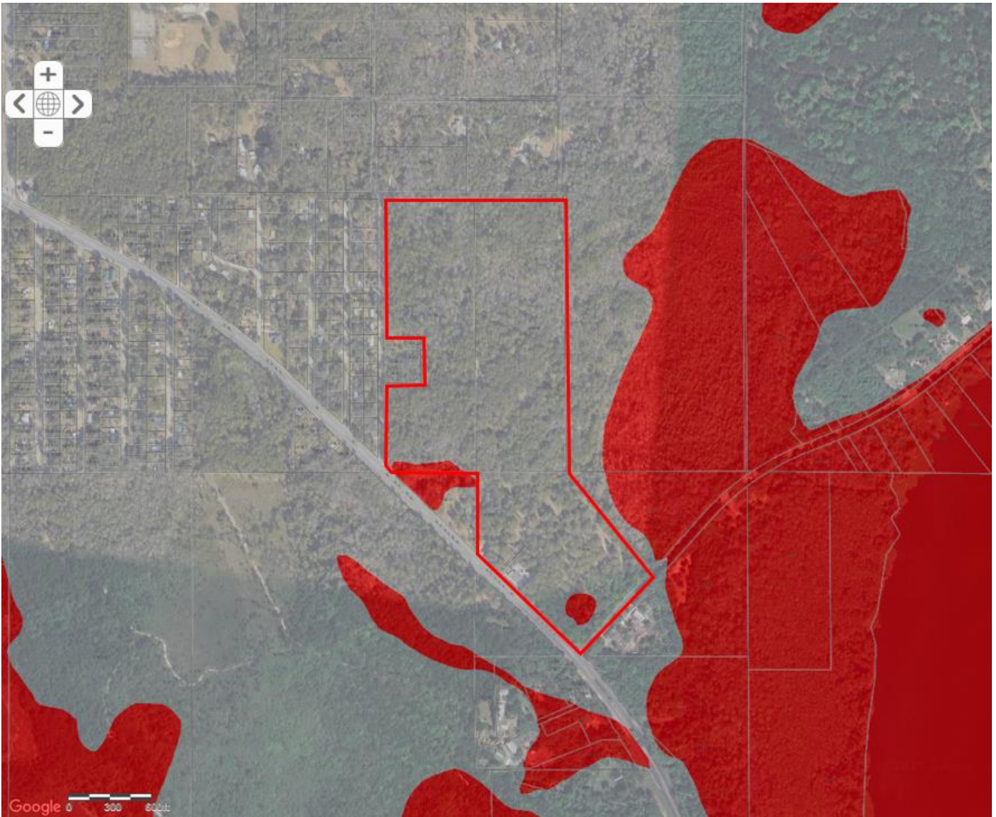
Figure 7: Flood Zone Map
