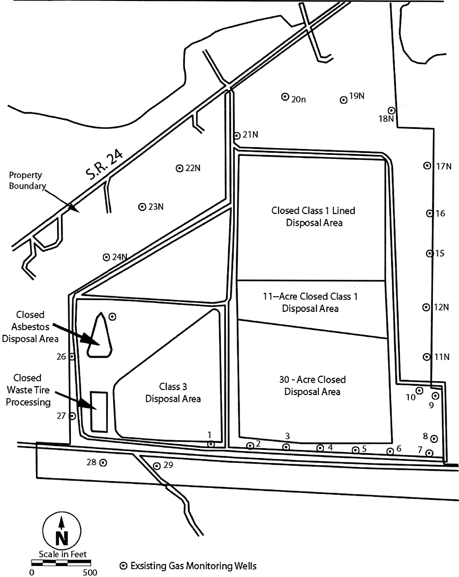
Figure 2 - Gas Probe Locations
